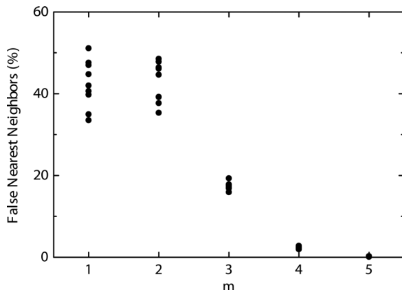
FIG. 2. Fraction of false nearest neighbors for different values of the external diffusivity as a function of the embedding dimension m . Calculations were performed using \tau = 1000 \Delta t , R_t = 15 , and L_2 -norm.
